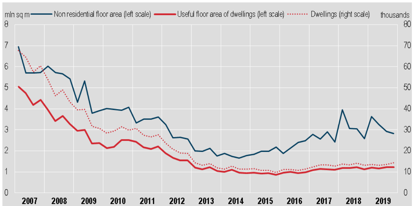
CHART 1. USEFUL FLOOR AREA OF DWELLINGS AND OF NON-RESIDENTIAL BUILDINGS, NUMBER OF DWELLINGS Q1 2007 – Q4 2019, seasonally adjusted, absolute values (a)
