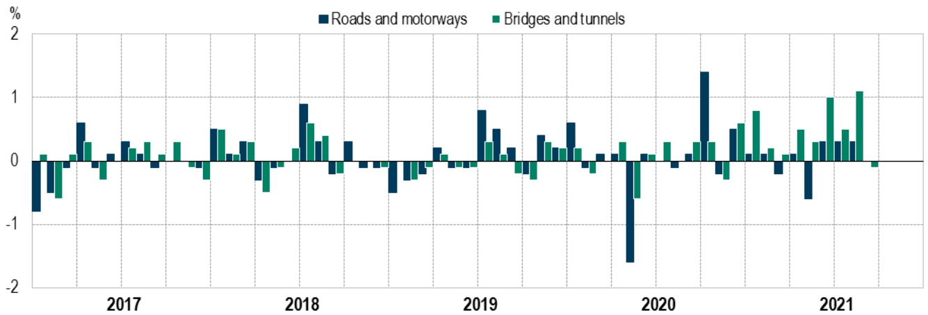
CHART 9. CONSTRUCTION PRODUCER PRICE INDEX, ROADS AND MOTORWAYS, BRIDGES AND TUNNELS January 2017 – September 2021, month on previous month percent changes (index, 2015=100)
