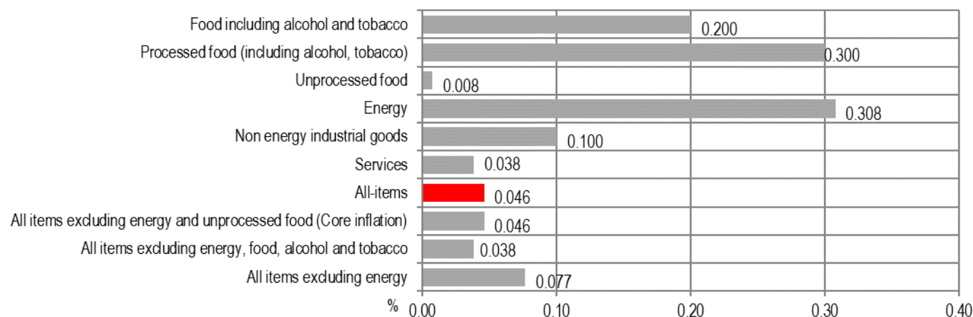
FIGURE 1. MEAN ABSOLUTE DEVIATION BETWEEN FLASH ESTIMATES AND HICP ANNUAL RATES. July 2020 – July 2021, percentage points
