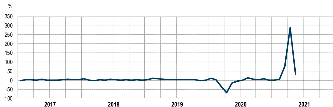
CHART 2. PRODUCTION IN CONSTRUCTION, MONTH ON SAME MONTH A YEAR AGO PERCENTAGE CHANGES January 2017 – May 2021, calendar adjusted data (index, 2015=100)
