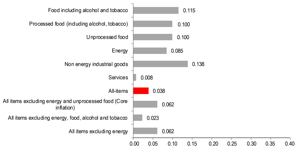
FIGURE 1. MEAN ABSOLUTE DEVIATION BETWEEN FLASH ESTIMATES AND HICP ANNUAL RATES. September 2016 - September 2017, percentage points
