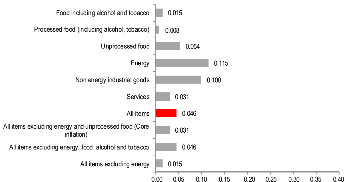
FIGURE 1. MEAN ABSOLUTE DEVIATION BETWEEN FLASH ESTIMATES AND HICP ANNUAL RATES. SEPTEMBER 2015-SEPTEMBER 2016, percentage points
